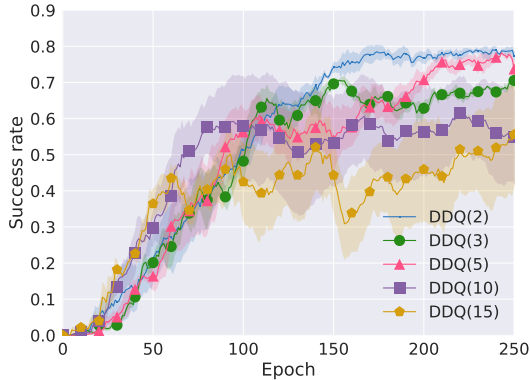
Figure 4: The learning curves of DDQ( K ) agents where (K - 1) is the number of planning steps.
