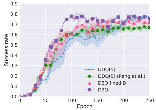
Figure 7: The learning curves of DDQ(5), DDQ(5) (Peng et al., 2018), D3Q fixed \theta_D , and D3Q agents.
