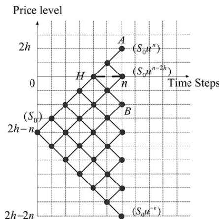
Fig. 5. Placing a CRR lattice on a grid for pricing a single-barrier option. A CRR lattice drawn in thick solid lines and circles is placed on a grid. The x -axis and the y -axis of this grid are denoted by thin solid lines. The coordinate of the root node of the CRR lattice is (0, 2h - n) . The barrier H is denoted by a thick dotted line. The values in parentheses denote stock prices.
