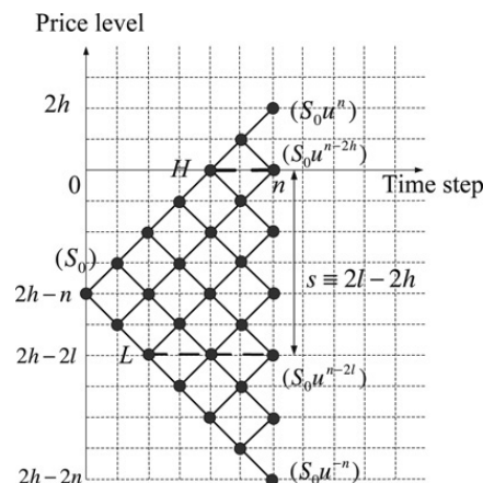
Fig. 7. Placing a CRR lattice on a grid for pricing a double-barrier option. A CRR lattice drawn in thick solid lines and circles is placed on a grid. The x -axis and the y -axis of this grid are denoted by thin solid lines. The coordinate of the root node of the CRR lattice is (0, 2h - n) . The two barriers H and L are denoted by thick dotted lines, and s denotes the distance between H and L . The values in parentheses denote stock prices.
