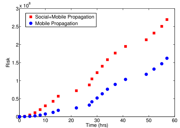
Fig. 5. Risk metric corresponding to Fig. 4: the accumulated infected population with respect to time. The results show clear tradeoffs between attack successfulness and risk of exposure.
