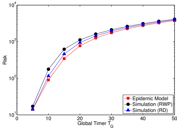
Fig. 3. Risk metric corresponding to Fig. 2. Epidemic models are capable of predicting both the attack successfulness and risk of exposure.
