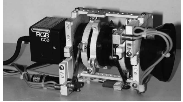
Fig. 5. This figure shows the motorized zoom lens used in our experiments, which is a Fujinon TV zoom lens H6 \times 12.5R with its aperture, zoom, and focus driven by three servo motors through pushrod links.
