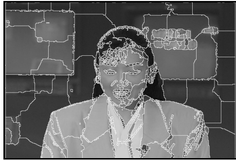
Experiment 4 (order-variant)
