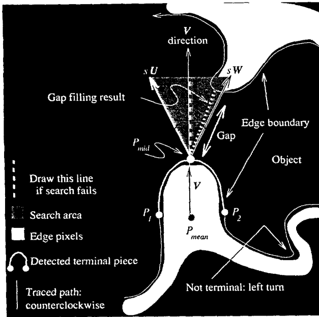
Fig. 15 Terminal extension algorithm. See text.
