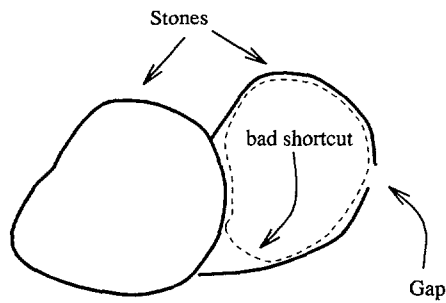
Fig. 2 Snake algorithm will fall into local minima in some cases.
