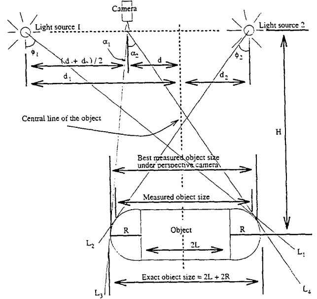
Fig. 18 Geometrical and radiometric model.
