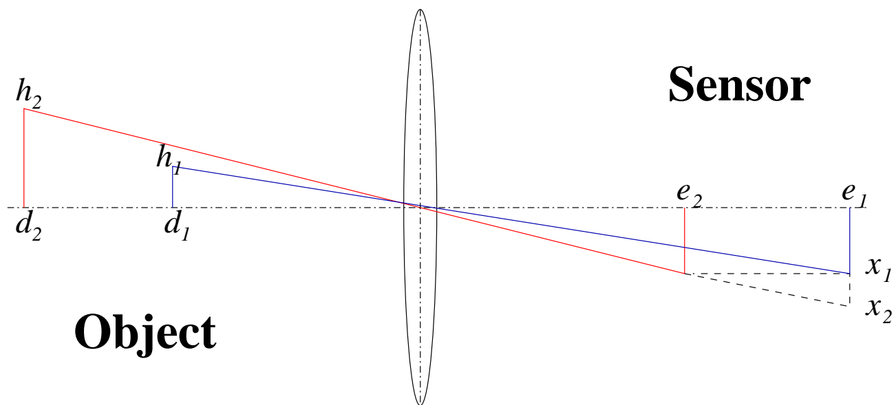
Figure 3: Camera geometry and parameters, where e_i is the effective focal length; d_i is the object distance; h_i is the actual object size; x_i is the size of camera sensor; and x_2 is the projection size of object 2 if it is focused on the same plane as where the object 1 is.
