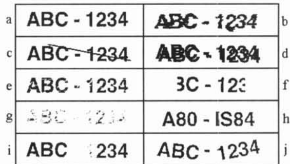
Figure 1: Main IC printed mark errors: (a) good, (b) smeared, (c) scraped, (d) double print, (e) broken, (f) missing ink, (g) bad contrast, (h) misprinted, (i) partial bad contrast, and (j) mis-orientation.
