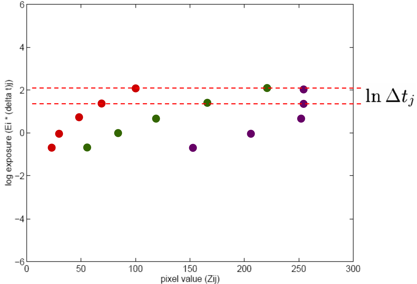
plot of g(Z_{ij}) from three pixels observed in five images, assuming unit radiance at each pixel
