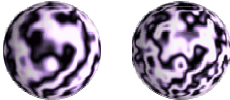
Standard 3 dimensional Perlin noise 4 octaves, persistence 0.25 and 0.5
