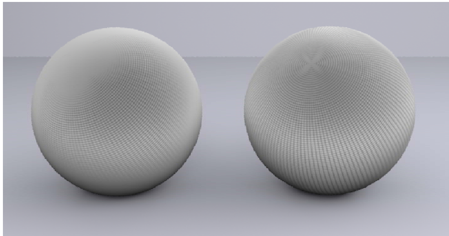
trilinear
