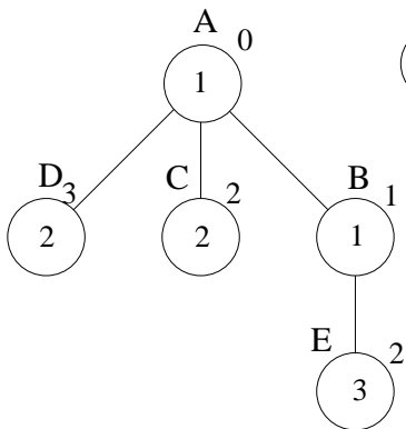
Figure 1: An broadcast tree for five processors.
