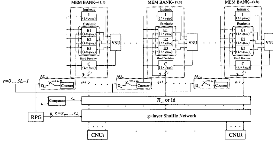
Figure 4: Elaborated (3, k) -regular LDPC decoder architecture.
