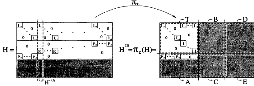
Figure 7: Structure of matrix \mathbf{H}^{en} .
