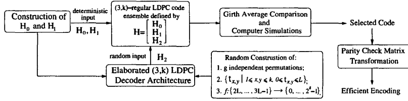
Figure 2: Joint design flow diagram.
