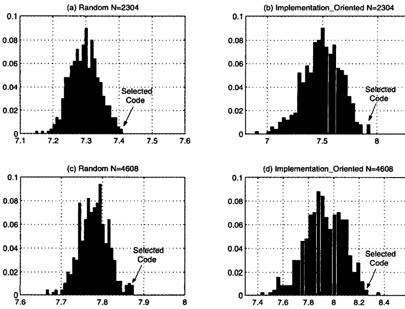
Figure 5: Histograms of girth average for (a)(c) fully random codes, and (b)(d) implementation-oriented codes.
