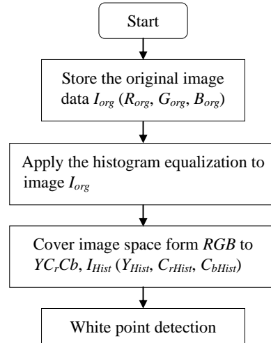
Fig. 3. Flowchart of white object purification.
