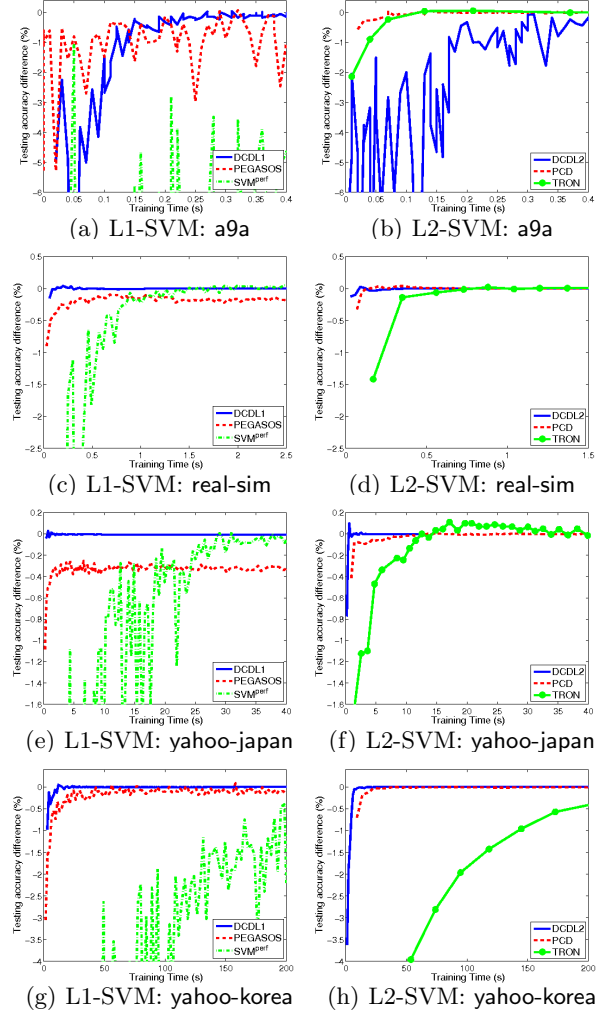
Figure 4. Time versus the difference of testing accuracy between the current model and the reference model (obtained using strict stopping conditions). Time is in seconds.
